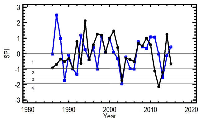
Fig. 1. The Standardized Precipitation Index for 12 month rainfall totals in 1986–2015 (Baborowko – blue, Grabow – black; Dryness categories acc. McKee et al. (1993): 1 – mild dryness (0 to -0.99), 2 – moderate dryness (-1 to -1.49), 3 – severe dryness (-1.5 to -1.99) and extreme dryness (<-2.0)
